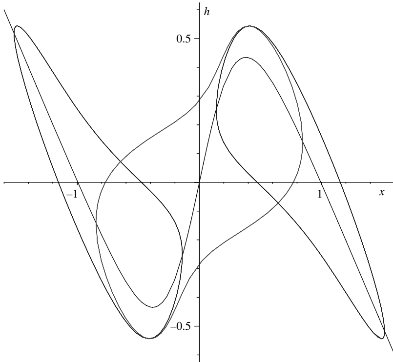
Figure 6. Three coexisting stable solutions of the Suzuki–Kubo equation for \beta=3 , \epsilon=0.05 and h=0.544 .
