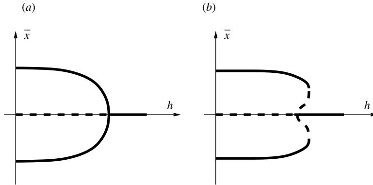
Figure 2. Two possible minimal scenarios of the emergence of a single periodic solution. Stable solutions are represented by solid lines, unstable are represented by dashed lines. In scenario (a), three solutions merge in a subcritical pitchfork bifurcation. In scenario (b), the central solution first undergoes a supercritical pitchfork bifurcation, emitting two unstable solutions. These unstable solutions disappear in fold bifurcations upon meeting the stable solutions.
