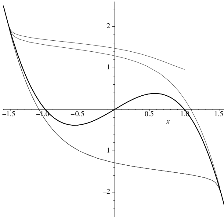
Figure 1. The picture of the (stable) hysteresis loop for large h . In this case, we take f(x) = x - x^3 , \epsilon = 0.05 and h = 2.0 .
