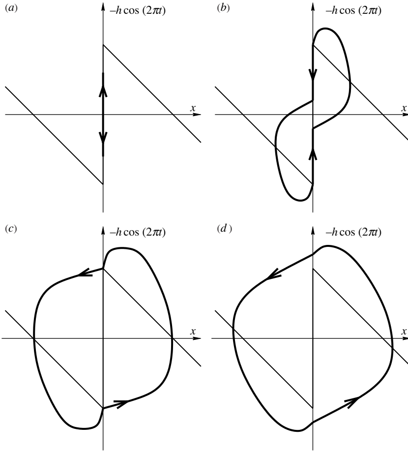
Figure 4. Evolution of the zero-mean solution of inclusion (4.8). (a) Solution is identically zero when h < 1 . (b) Growth of nontrivial parts when 1 < h < h_{cs} . (c) The solution experiences a bifurcation at h = h_{cs} when the trivial parts, where x(t) = 0 on an open interval, disappear completely. (d) The stable solution for h > h_{cs} contains no trivial parts.
