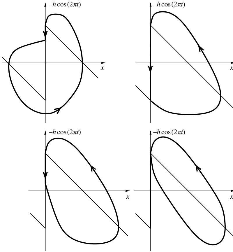
Figure 5. The evolution of the right unstable solution until its annihilation at h = h_{ca} .
