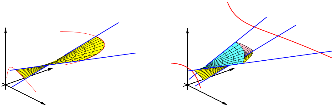
FIGURE 1. Cremona-convex hulls
