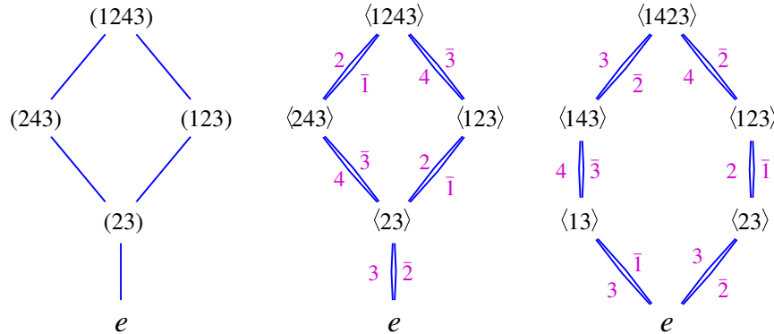
FIGURE 9. Conjugation by \gamma on labeled intervals.
