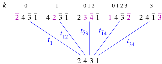
FIGURE 3. Covers of 2\ 4\ \bar{3}\ \bar{1} .
