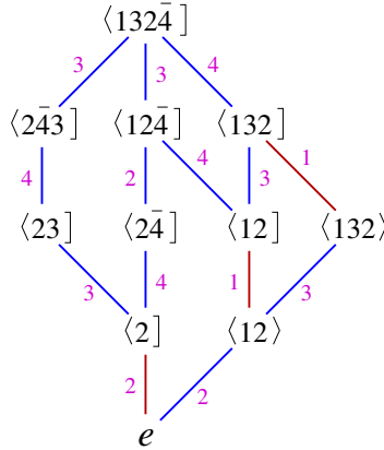
FIGURE 6. The interval [e, \langle 132\bar{4} \rangle]_{\prec} .
