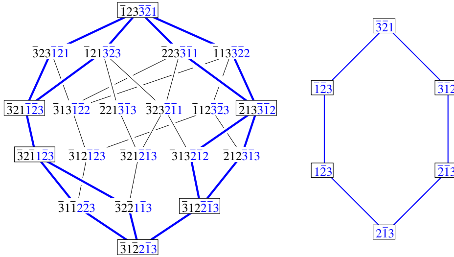
FIGURE 4. The intervals [\bar{3}1\bar{2}2\bar{1}3, \bar{1}23\bar{3}\bar{2}1]_{\triangleleft_0} and [2\bar{1}3, \bar{3}\bar{2}1]_0 .
