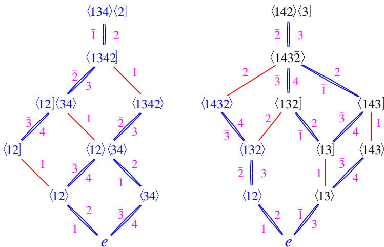
FIGURE 8. Conjugation by \rho on labeled intervals.
