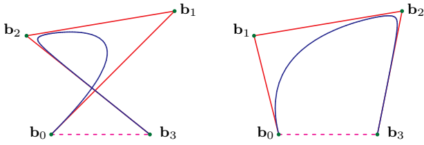
Fig. 8. Rational cubic Bézier planar curves with t = 5 .
