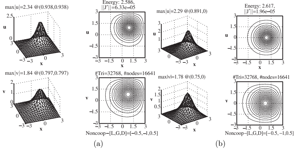
FIGURE 8. Profiles and contours of two asymmetric positive solutions (a) and (b) to system (4.25) with \lambda = -0.5 , \gamma = -1 , \delta = 0.5 , \Omega = (-3, 3) \times (-3, 3) .
