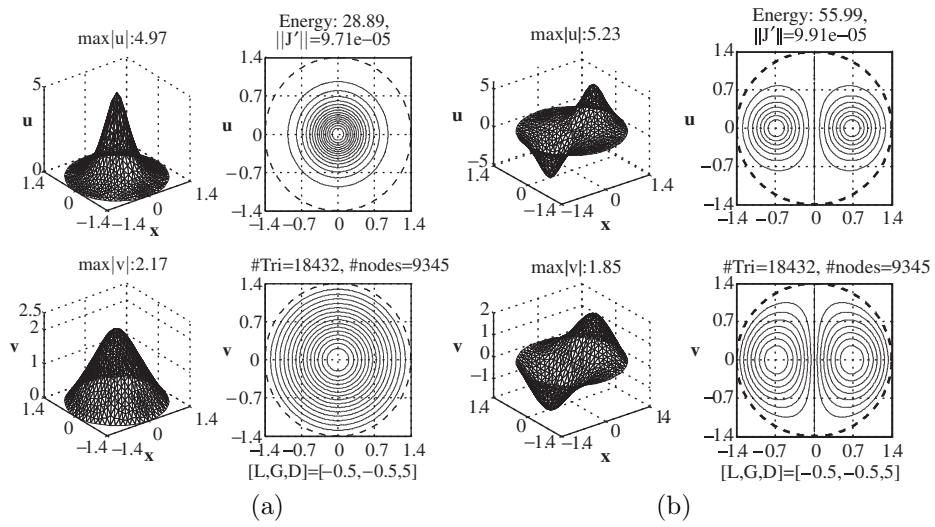
FIGURE 4. Profiles and contours of a positive solution (u_1, v_1) (a) and a 2-peak sign-changing solution (u_2, v_2) (b) where L = \text{span}\{u_1\} \times \text{span}\{v_1\} to system (4.2) with p = q = 3, \lambda = \gamma = -0.5, \delta = 5 . The dashed circle indicates the boundary of the domain.
