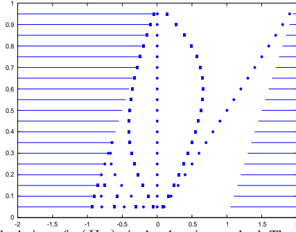
Figure 4: Our recalculation of \sigma(H_+) via the shooting method. The eigenfunction corresponding to \lambda = 2\omega has been found in the explicit form, confirming our plot. Bifurcation at \omega \approx 0.5 is absent. Our recalculation of \sigma(H_-) coincides with the right plot on Figure 3 obtained by [CP06].
