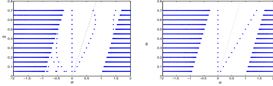
Figure 3: Spectra of H_+ (left) and of H_- (right) versus \omega , computed in [CP06] via Scalapack library on a parallel computer cluster. Note the absence of the exact eigenvalue \lambda = 2\omega of \sigma(H_+) . These plots are courtesy of [CP06].
