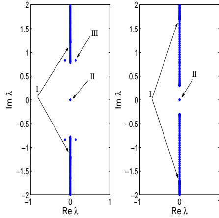
Figure 6: Spectra of L_\omega at \omega = 0.2 (left) and \omega = 0.7 (right), computed in [CP06] via Scalapack library on a parallel computer cluster. Note the absence of exact eigenvalues \lambda = \pm 0.4i on the left plot. These plots are courtesy of [CP06].
