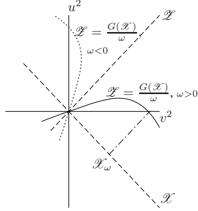
Figure 1: Existence of solitary waves in the coordinates \mathcal{X} = v^2 - u^2 , \mathcal{Z} = v^2 + u^2 . Solitons with \omega > 0 and \omega < 0 correspond to the bump on the v^2 axis and to the dotted bump on the u^2 axis (respectively) in the first quadrant.
