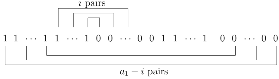
Figure 3: non-crossing pairings of 1^{a_1}0^{a_1}1^{a_2}0^{a_2} .
