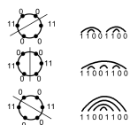
Figure 2: The corresponding regions and pairings of the binary string (1^2 0^2)^2 .
