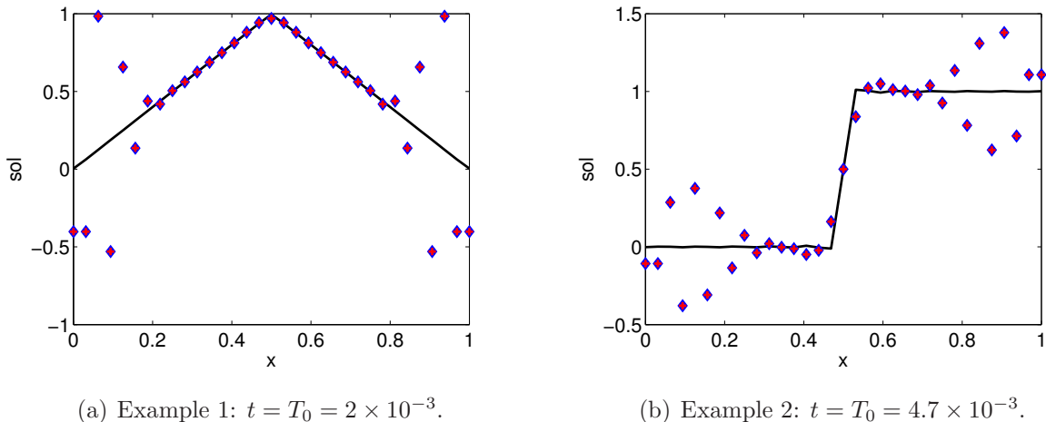
Figure 2: Comparison of exact (solid line) and numerical solutions (Euler in diamonds and CN in plus, they are on the top of each other) at fixed time for the two examples.
