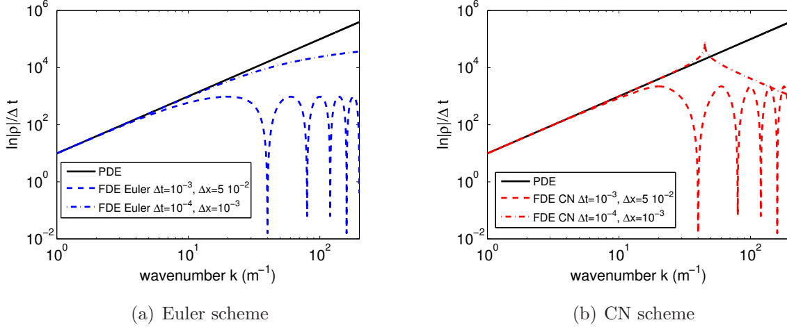
Figure 1: Comparison in log–log scale of dispersion relations for the PDE and numerical schemes at various values of space and time steps. FDE stands for “Finite Difference Equation”. Note the singularity at k_u = 45.05 of the Crank-Nicolson FDE for \Delta t = 10^{-4} and \Delta x = 10^{-3} .
