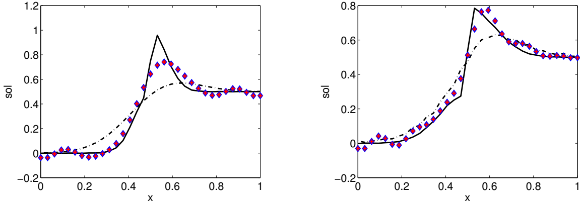
(a) Case without noise: t = T_0 = 1 , k_d = 10 .
