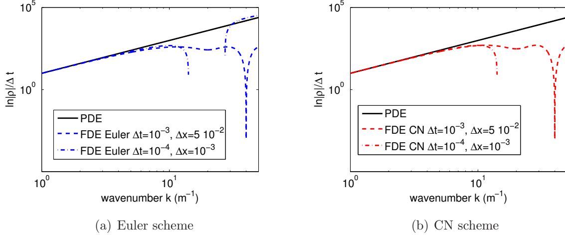
Figure 12: Comparison in log–log scale of the exact ( \omega versus k ) and numerical ( |\rho|/\Delta t versus k ) dispersion relations for the regularized problem for several values of space and time steps. For these plots \nu = 1 and k_d = 10 .
