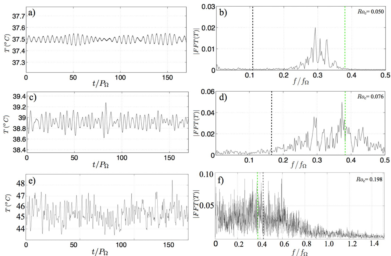
Figure 18. Thermistor T_3 temperature time series (left column) and corresponding Fourier spectra (right column) from the \Gamma = 1.87 , E = 2 \times 10^{-5} RC laboratory cases (a,b) RC_l^1 ; (c,d) RC_l^2 ; and (e,f) RC_l^3 . Time is reported in rotation periods, P_{\Omega} , in panels a, c and e. Frequency is normalized by the rotation frequency f_{\Omega} in panels b, d and f. The vertical dashed black lines denote each case's normalized LSC frequency, f_{LSC}/f_{\Omega} \simeq 2.2Ro_c . The vertical dashed green lines denote the normalized onset frequency, f^O/f_{\Omega} , for oscillatory convection with no-slip boundaries [38,83].
