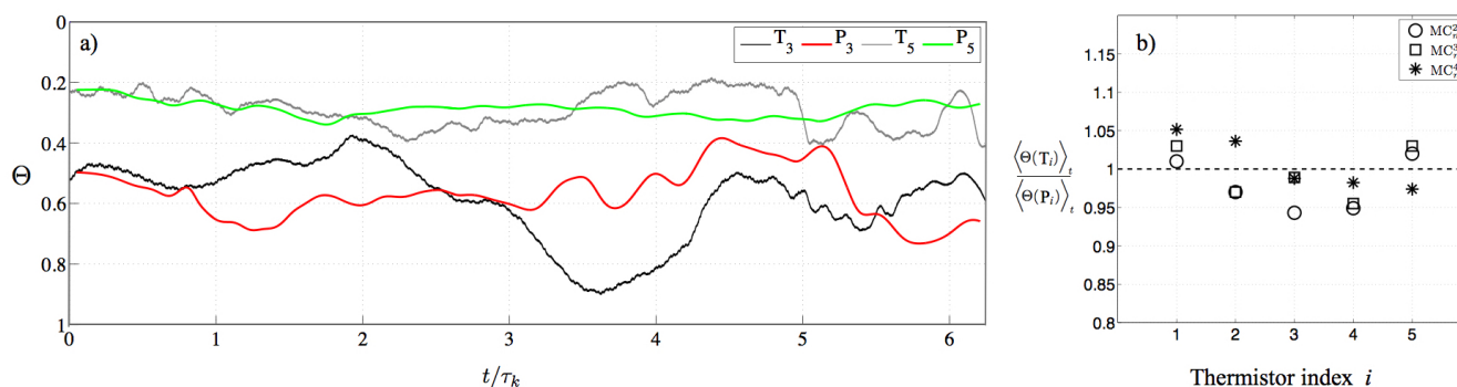
Figure 11. (a) Temperature time series acquired on thermistors T_3 and T_5 in the MC_l^2 experiment ( \Gamma \simeq 3.92 ; Ra = 6.46 \times 10^4 ; N = 2.24 ) with temperature normalized by \Delta T , and the corresponding time series of the non-dimensional temperatures measured on the point probes P_3 and P_5 in numerical simulation MC_n^2 ( \Gamma \simeq 4 ; Ra = 6.47 \times 10^4 ; N = 2.18 ); (b) Time-averaged, non-dimensional temperature on each thermistor (i.e., \Theta(T_i) for the i^{th} thermistor), normalized by the time-averaged, non-dimensional temperature of the corresponding numerical point-probe ( \Theta(P_i) ).
