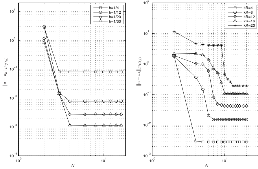
Figure 4: Log-log plot of errors in L^2 -norm vs the truncation order N for R_0 = 0.5 , R = 1 and kR = 4 (left); The correlation between the truncation order N and the parameter kR as h = 1/15 (right).
