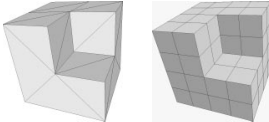
FIGURE 5. Fichera corner: initial meshes.
