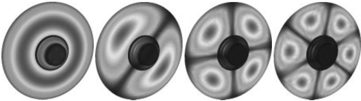
FIGURE 6. Accelerator induction cell: eigenfunctions 1, 2, 4 and 8.
