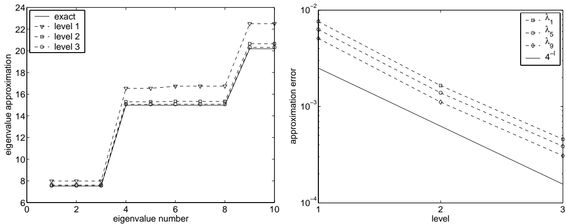
FIGURE 4. Unit sphere: eigenvalue convergence.
