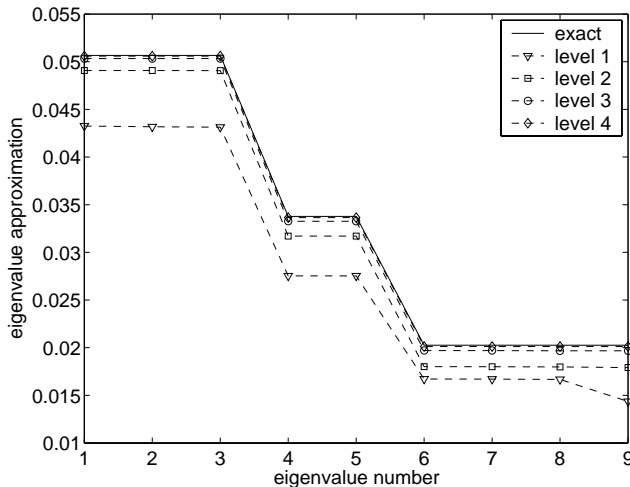
FIGURE 1. Unit cube: eigenvalue convergence.
