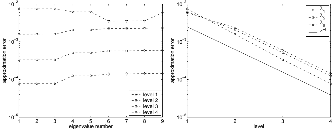
FIGURE 2. Unit cube: approximation error.
