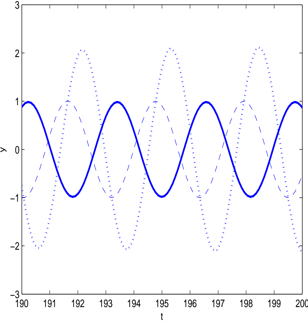
Exact Solution with y_0 and y_0 + \varepsilon y_1
