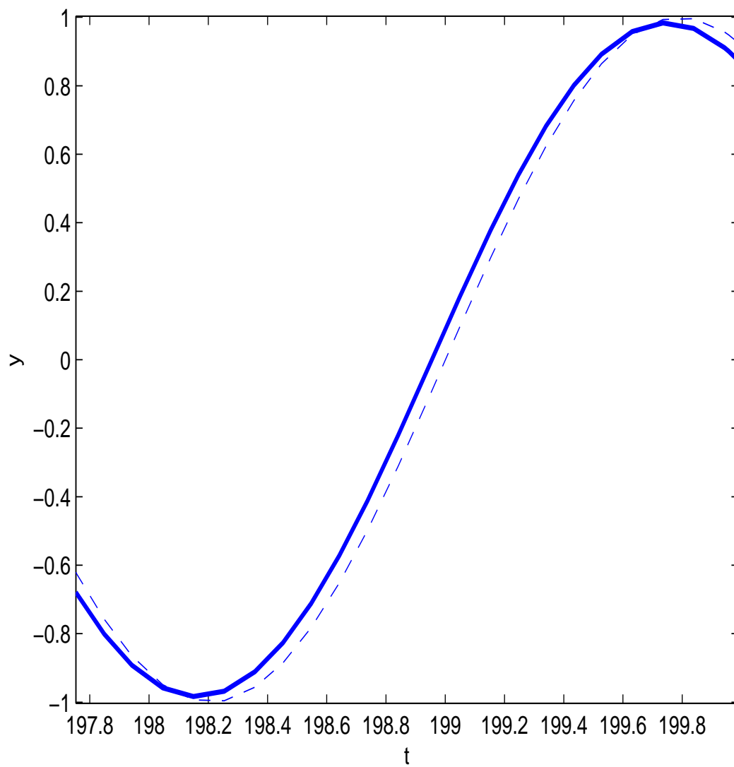
Exact Solution with p_0
