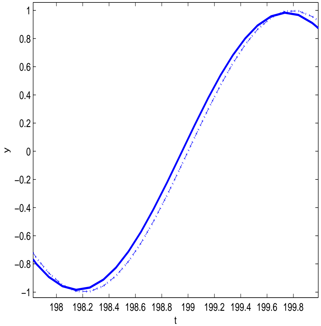
Exact Solution with p_0 and p_0 + \varepsilon p_1
