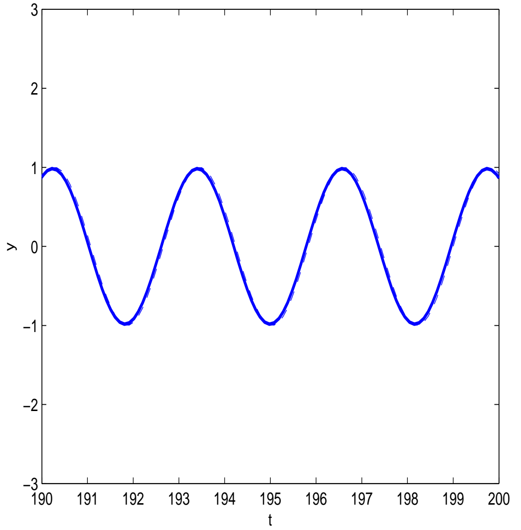
Exact Solution with p_0
