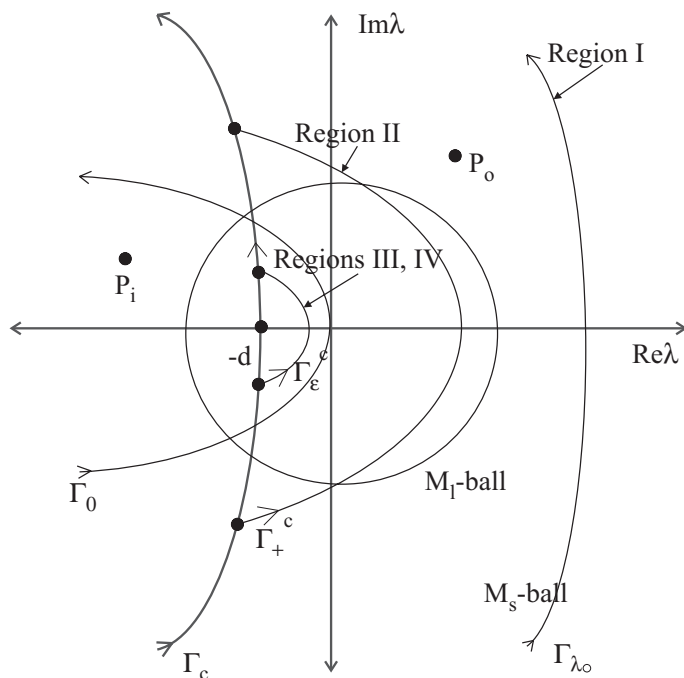
Figure 2. Contours in the complex plane
