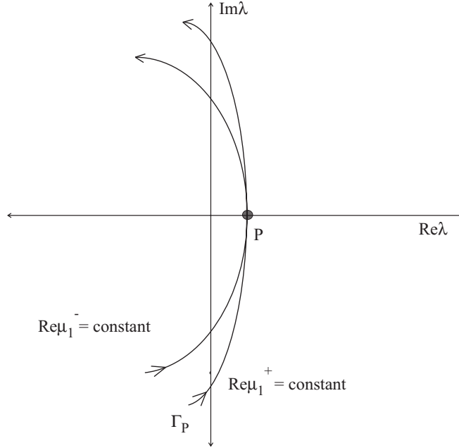
Figure 4. The contours of Lemma 4.1.
