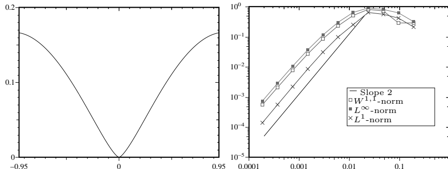
FIGURE 1. (Left) Graph of u_{\text{visc}} . (Right) Convergence tests.
