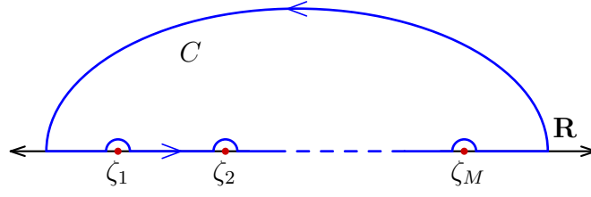
FIGURE 1. Contour in upper half plane
