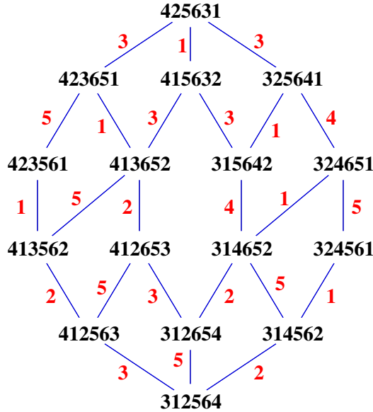
FIGURE 2. The interval [(3, 1, 2, 5, 6, 4), (4, 2, 5, 6, 3, 1)]_4 .
