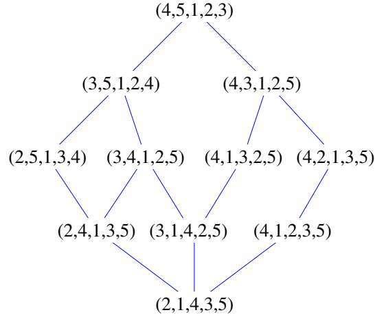
FIGURE 1. The interval [(2, 1, 4, 3, 5), (4, 5, 1, 2, 3)]_2 .
