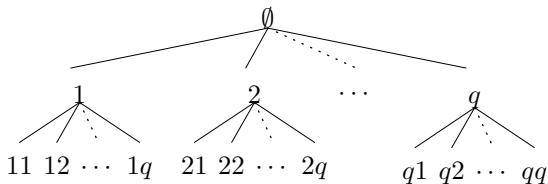
The tree \mathcal{T}^{(q)}
