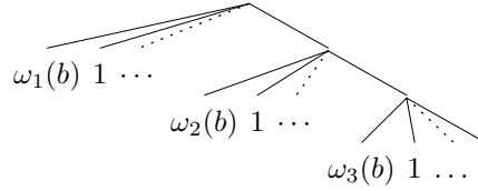
The automorphism b_\omega \in G_B
