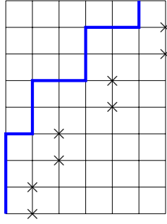
FIGURE 2. Lattice path corresponding to the images (1, 1, 1, 2, 2, 4, 4, 6) with x = 6 . The stars indicate the right boundary (1, 1, 2, 2, 4, 4, 6, 6) .
