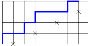
FIGURE 1. Lattice path corresponding to the sequence (1, 3, 4, 7) with x = 8 . The stars indicate the right boundary (1, 3, 5, 7).
