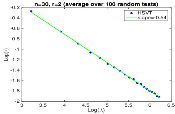
Figure 3: Recovery error \epsilon := \|\mathbf{X} - \widehat{\mathbf{X}}\|_F vs oversampling factor \lambda for the procedure (58)
