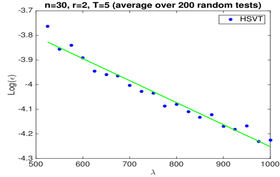
Figure 4: Recovery error \varepsilon := \|\mathbf{X} - \widehat{\mathbf{X}}\|_F vs oversampling factor \lambda for the procedure (69)-(70)-(71)
