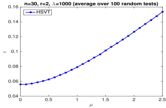
Figure 2: Recovery error \varepsilon := \left\| \mathbf{X} - \frac{\mathbf{X}^{\text{ht}}}{\|\mathbf{X}^{\text{ht}}\|_F} \right\|_F vs magnitude \mu := \|\mathbf{e}\|_1 of prequantization error
