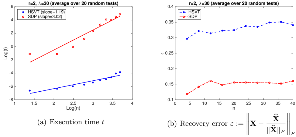
Figure 1: Comparison of the procedures (22) and (35) when the dimension n varies
